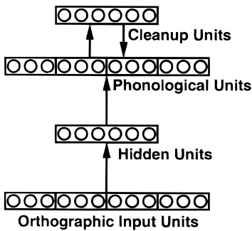
FIG. 1. Model architecture used in all simulations.
