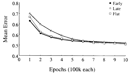
FIG. 5. Performance in the Flat condition (Simulation 2) compared to the same items in the Early and Late conditions in Simulation 1.
