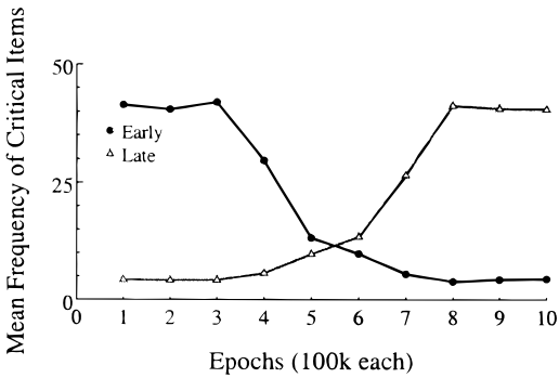
FIG. 2. Frequency trajectories of critical items in Simulation 1.
