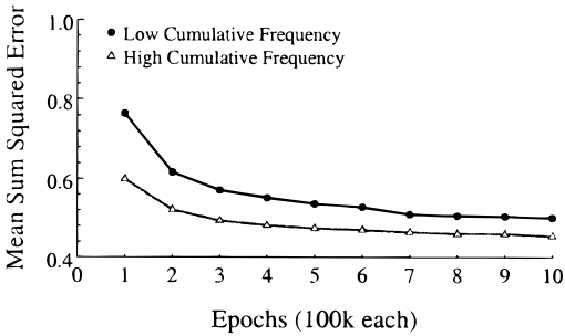
FIG. 6. Performance on high and low cumulative frequency items within the Flat condition.
