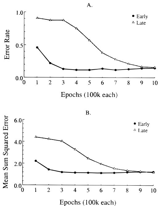
FIG. 4. Performance over time for Simulation 2: (A) error rate and (B) sum squared error.
