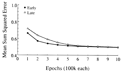
FIG. 3. Performance over time for critical items in Simulation 1.
