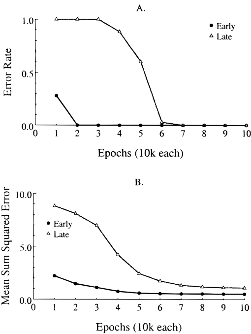
FIG. 7. Performance over time for critical items in Simulation 3: (A) error rate and (B) sum squared error.
