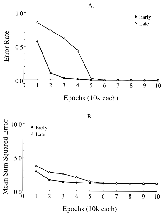
FIG. 8. Performance over time for critical items in Simulation 4: (A) error rate and (B) sum squared error.
